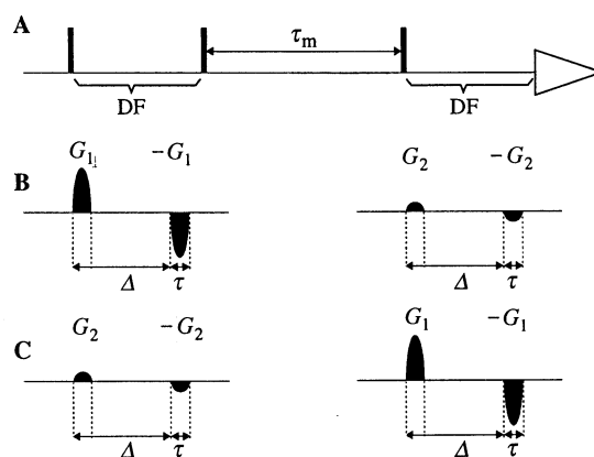
Fig. 2 (A) Schematic survey of a one-dimensional transient NOE experiment with diffusion filters. The three vertical bars represent 90° hard pulses at the ^1\text{H} frequency. The initial 180° pulse of the transient NOE experiment 31 is decomposed into two 90° pulses which enclose the first diffusion filter. The second diffusion filter is inserted between the observation pulse and the start of data acquisition. (B) and (C) Diffusion filters, which consist of two pulsed field gradients (PFG) of length \tau spaced by the diffusion time \Delta . The strength of the PFGs is represented by the height of the symbol. The HYDRA-N experiment for selective observation of hydration water molecules consists of the difference between two recordings of (A) which use the arrangements of the diffusion filters shown in (B) and (C), respectively, and otherwise identical conditions.
