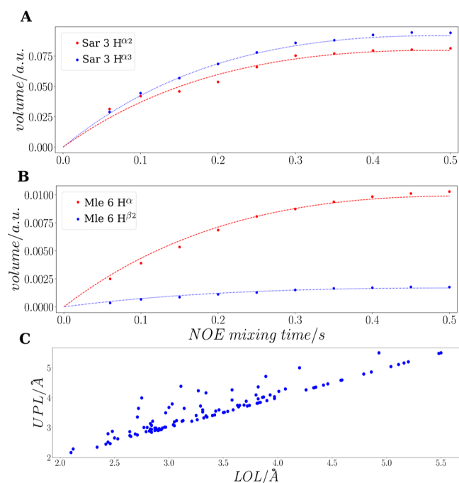
Figure 3. eNOE buildup data for the geminal protons H α2 , H α3 of Sar 3 (A) and H α , H β2 of Mle 6 (B) (CsA in CDCl 3 / n -hexadecane- d 34 ) are shown. The buildup (dotted lines) curves were fitted to the data according to eq 3. For Mle 6, the obtained restraints are r_{ij} = 3.61 Å and r_{ji} = 2.69 Å. Differing restraints are due to normalization to different diagonal-peak volumes, V_{ii} = 1.029 \times 10^{12} (H β2 , blue curve) and V_{jj} = 2.051 \times 10^{11} (H α , red curve). V_{ii} is significantly larger than V_{jj} because of signal overlap, which cannot be resolved by deconvolution. In contrast, for Sar 3, V_{ii} = 7.087 \cdot 10^{10} (H α3 , blue curve) and V_{jj} = 7.340 \cdot 10^{10} (H α2 , red curve), which results in r_{ij} = 1.80 Å and r_{ji} = 1.76 Å. To take into account possible errors in volume determination, we have, therefore, set the upper and lower limit distance limits (UPL and LOL) to \max(r_{ij}, r_{ji}) and \min(r_{ij}, r_{ji}) , respectively. The correlation time, \tau_c = 0.47 ns, for restraint generation was determined as described in the main text. Deviations of the restraints r from the fixed distance between geminal protons, r = 1.72 Å, can be attributed to local variations in \tau_c . (C) Lower- and upper-limit distance restraints are shown before the correction is applied for methyl groups. The NOESY data have been acquired with a relaxation delay of 10 s to allow for complete relaxation prior to the next scan.
