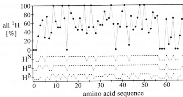
Fig. 4. Assignment with GARANT for the mutant homeodomain Antp (C39S,W56S) when using automated peak picking for obtaining the observed peaks, and the 3D NMR structure of Antp (C39S) as a source of supplementary input data. 2D ^1\text{H} TOCSY and NOESY spectra recorded in \text{H}_2\text{O} and a TOCSY spectrum recorded in \text{D}_2\text{O} were used as the primary data. All spectra were recorded at 10 °C, protein concentration 1.5 mM, pH 4.3. The TOCSY spectrum in \text{D}_2\text{O} was recorded at 500 MHz on a Bruker AMX spectrometer, the spectra in \text{H}_2\text{O} at 750 MHz on a Varian Unity-plus spectrometer. The same presentation as in Fig. 3A is used.
