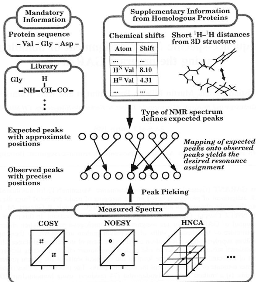
Fig. 1. The general concept of the program GARANT for automated sequence-specific NMR assignment of proteins. Boxes at the top represent the sources upon which prediction of expected peaks is based. The two boxes in the upper left represent mandatory information that is provided by a program library and by the amino acid sequence. The box in the upper right lists supplementary information that may be obtained from homology considerations. The box at the bottom represents the experimental NMR spectra from which the observed peak positions are extracted. The central part of the drawing indicates the search for optimal mapping of expected and observed peaks, which eventually yields the desired assignments (see text).
